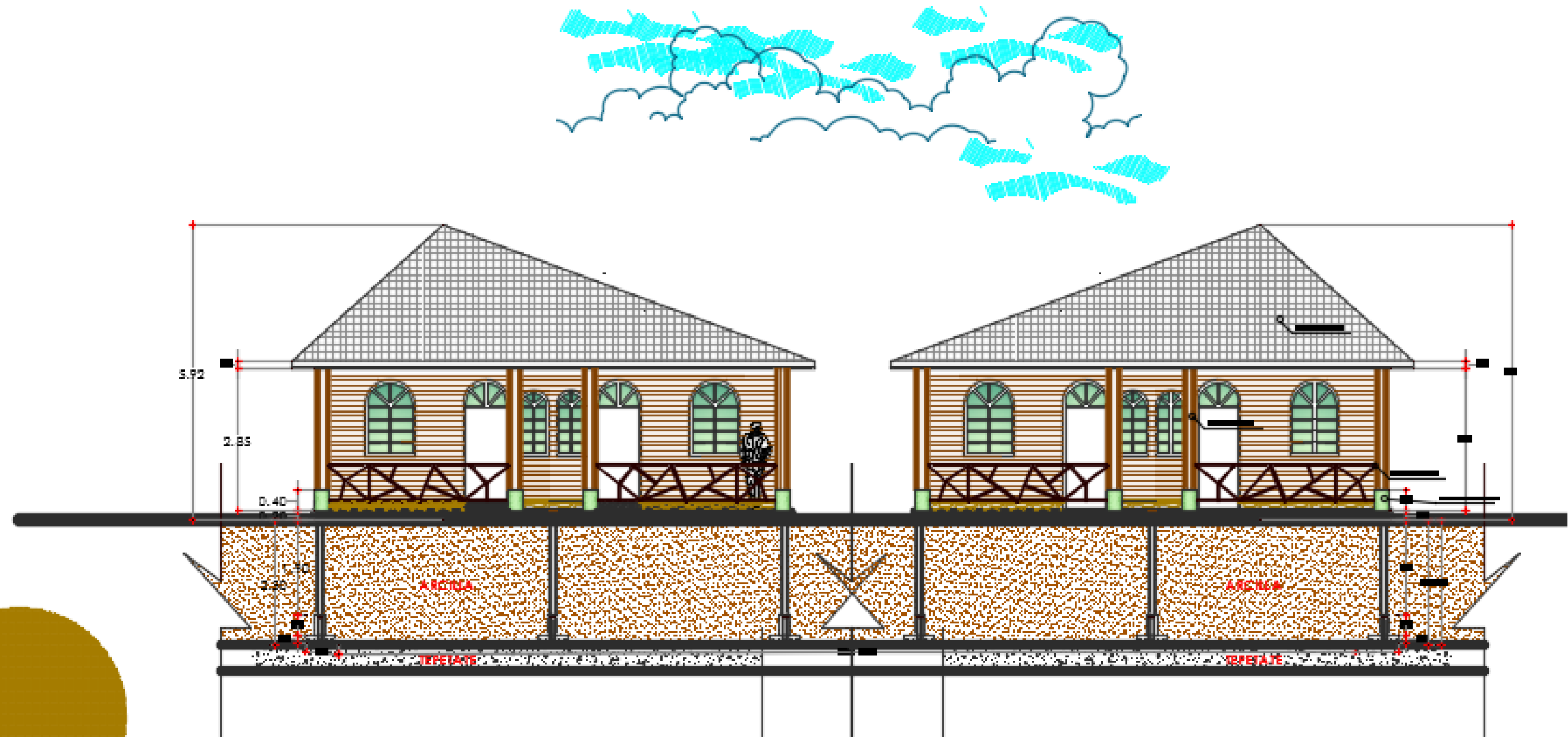
ALZADO PRINCIPAL
